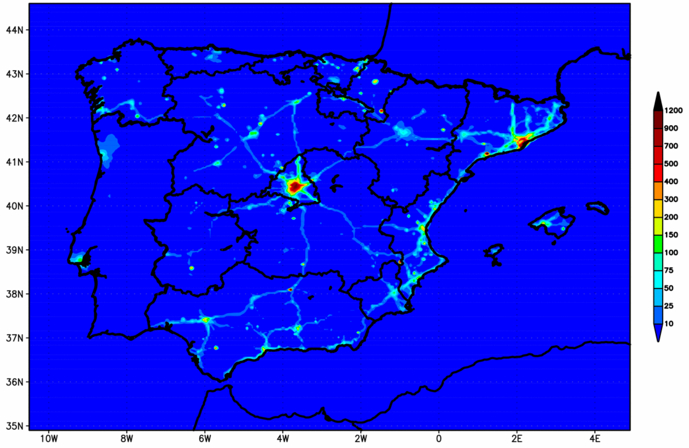
BSC-ES/HERMES Emissions NO (mole/h) 00z 26 FEB 07 - Iberian Peninsula Res:4x4km
